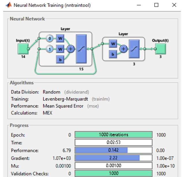
Fig. 9: Training window of Elman backpropagation
