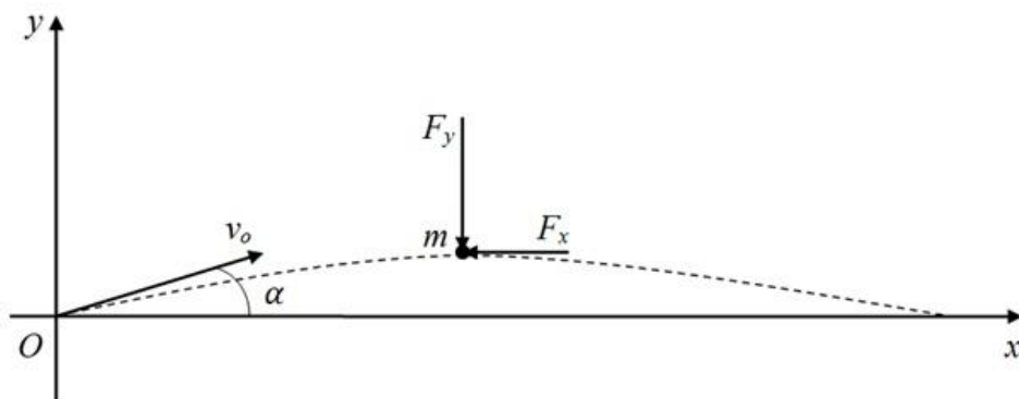
Fig. 3. Calculation scheme of MV [6]
